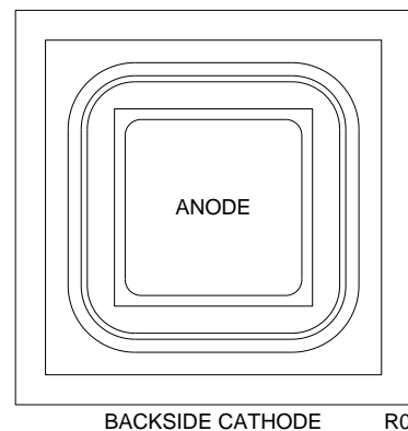
Figure 3. CPZ59X Chip Geometry (new)
