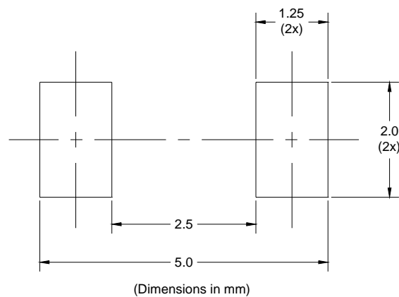
Figure 3: SOD-80 Mounting Pad Geometry
