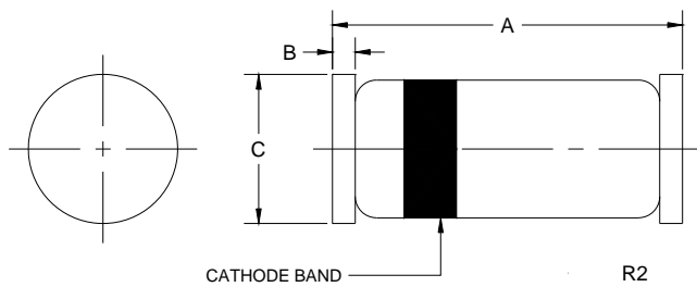
Figure 1: SOD-80 Mechanical Outline
